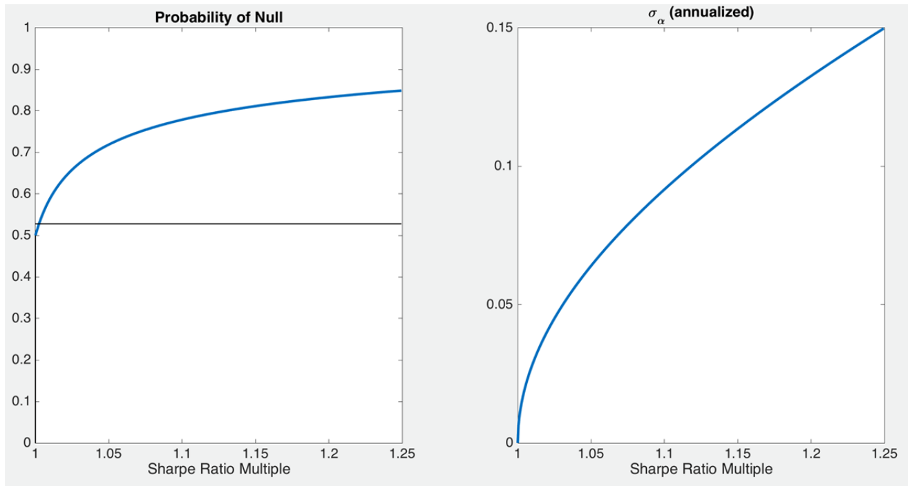
Figure 5: UMD is redundant in relation to the model {Mkt SMB ROE IA}. Bayesian intercept test for UMD. Sample 1972-2013. Horizontal axis: Sharpe ratio for the alternative as a multiple of the ratio under the null hypothesis (latter is 0.44 or 3.9 times the Market Sharpe ratio).
