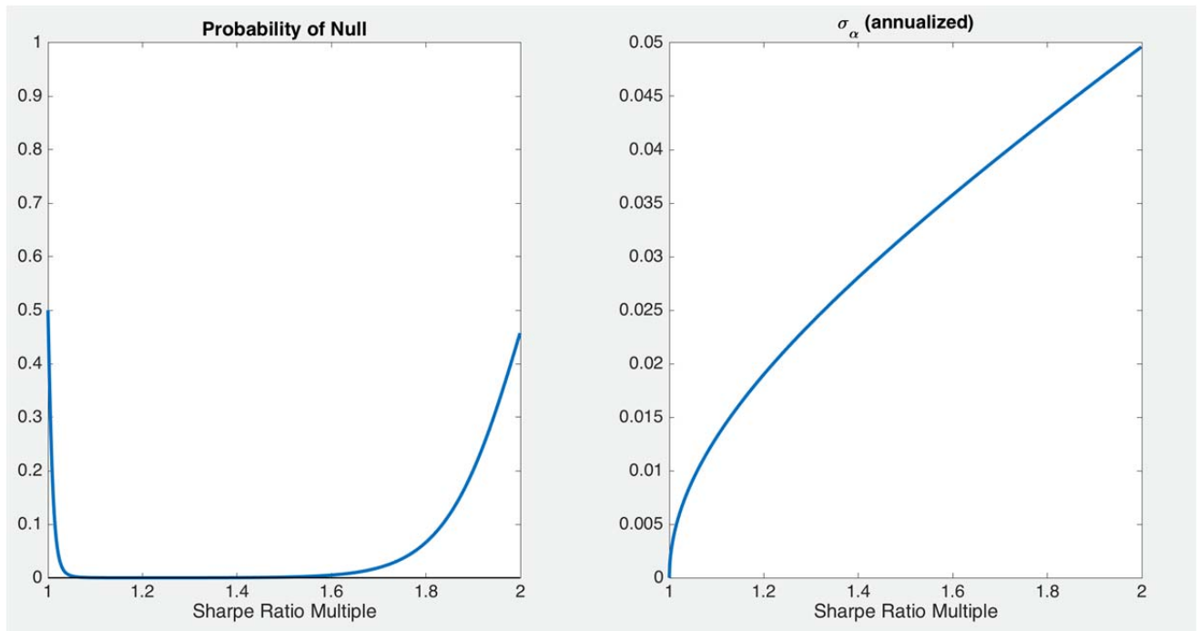
Figure 8: Sample 1972-2013, Model = {Mkt SMB IA ROE UMD HML m }. Test assets: 25 Book-to-market/investment portfolios. Horizontal axis: Sharpe ratio for the alternative as a multiple of the ratio under the null hypothesis (latter is 0.50 or 4.8 times the Market Sharpe ratio).
