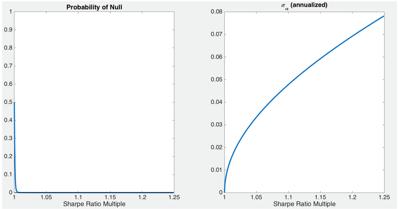
Figure 4: HML^m is not redundant in relation to the other factors \{Mkt\ SMB\ ROE\ IA\ UMD\} in the top model. Bayesian intercept test for HML^m . Sample 1972-2013. Horizontal axis: Sharpe ratio for the alternative as a multiple of the ratio under the null hypothesis (latter is 0.44 or 3.9 times the Market Sharpe ratio).
