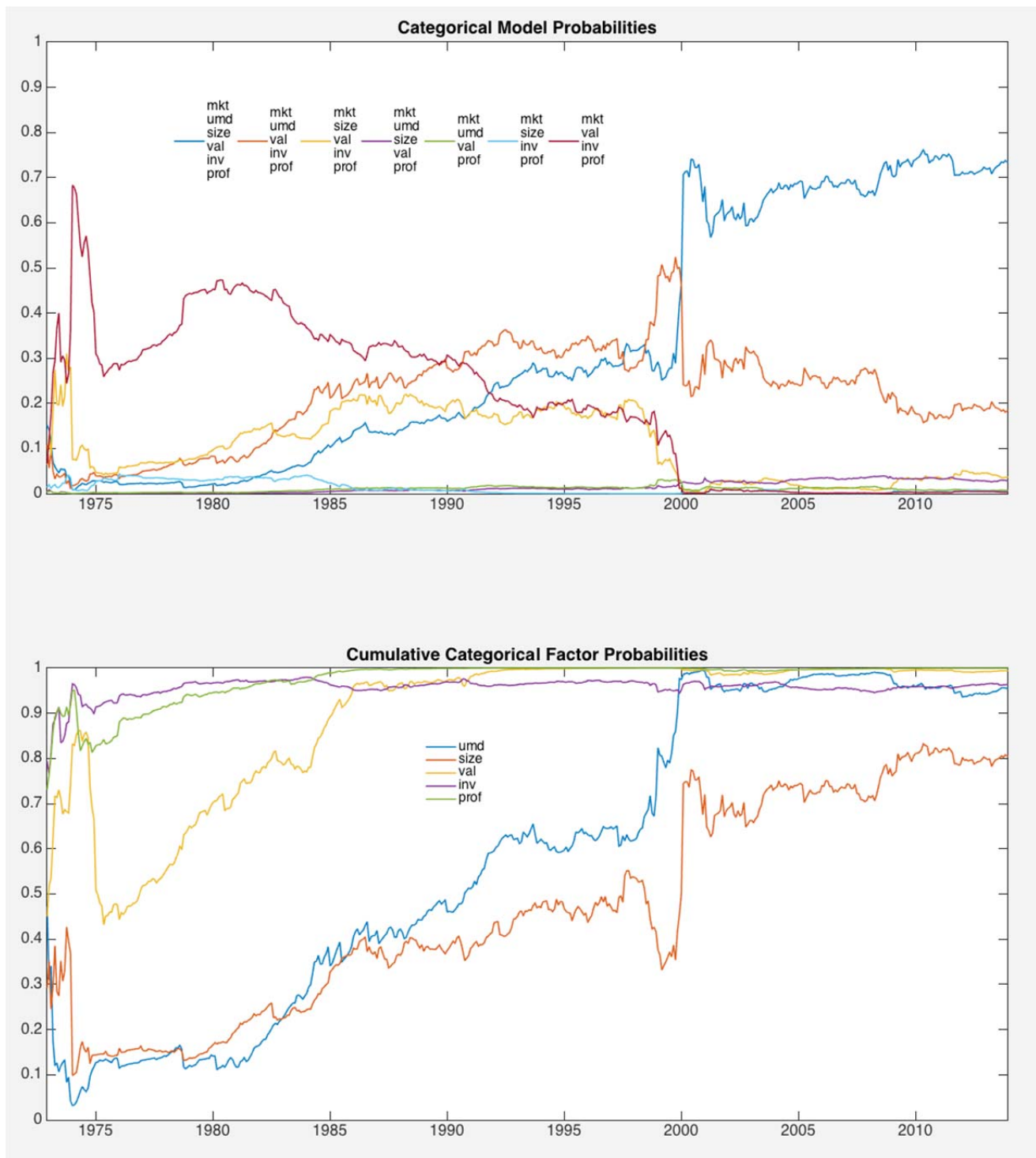
Figure 3: Sample 1972-2013, Sh_{\max} = 1.5 \times Sh(\text{Mkt}) .
