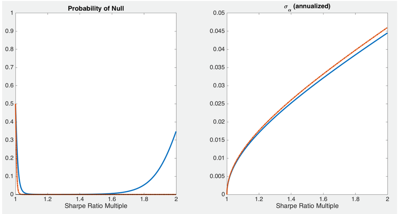
Figure 6: Sample 1972-2013, Model = {Mkt ME IA ROE}. Test assets = 25 size-momentum portfolios (blue line) plus UMD, HML^m (red line). Sample 1972-2013. Horizontal axis: Sharpe ratio for the alternative as a multiple of the ratio under the null hypothesis (latter is 0.43 or 3.8 times the Market Sharpe ratio).
